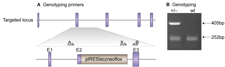
Figure 2: Genotyping details
