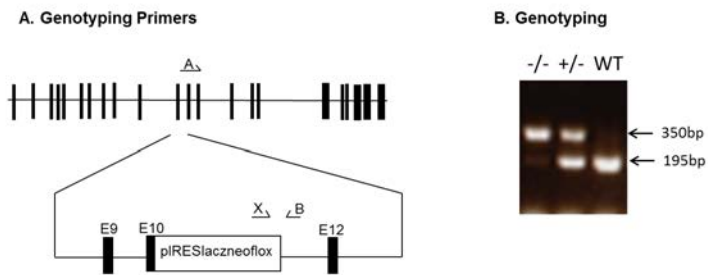
Figure 2: Genotyping details
