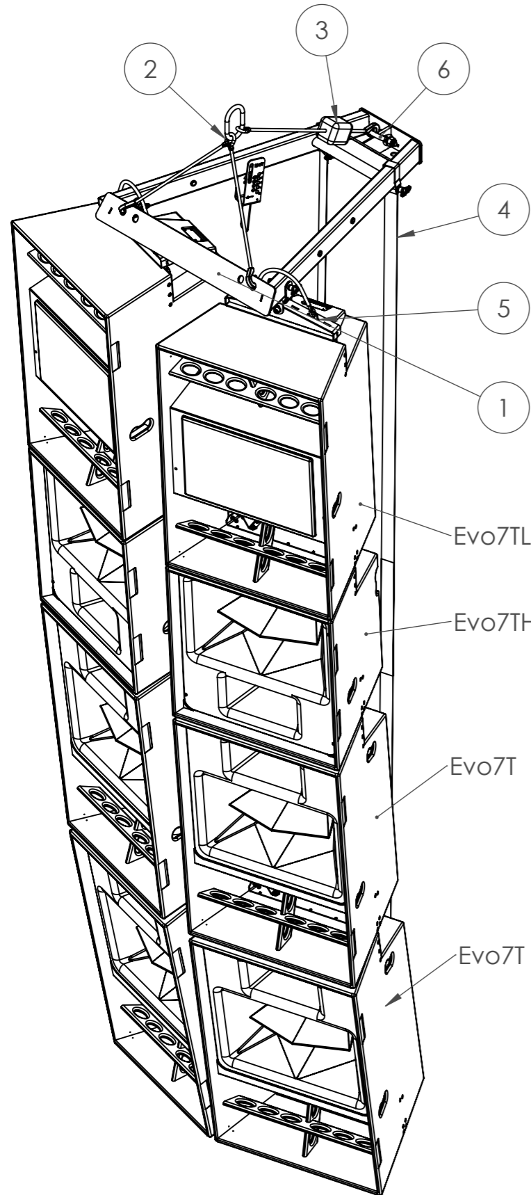
Example Array - Speakers not included in accessory kit.
